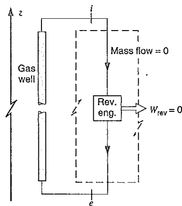
FIGURE 15.2 Illustration showing the relation between reversible work and the criteria for equilibrium.
