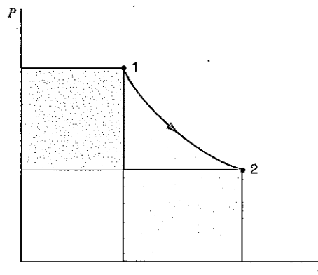
FIGURE 11.1 Comparison of shaft work and boundary-movement work.
