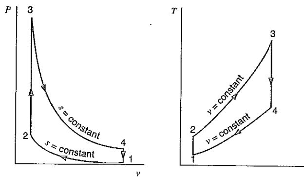
FIGURE 11.28 The air-standard Otto cycle.
