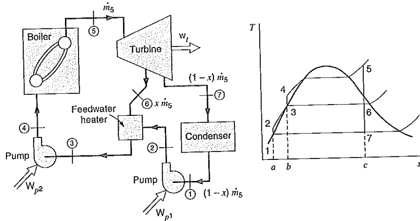
FIGURE 11.10 Regenerative cycle with open feedwater heater.
