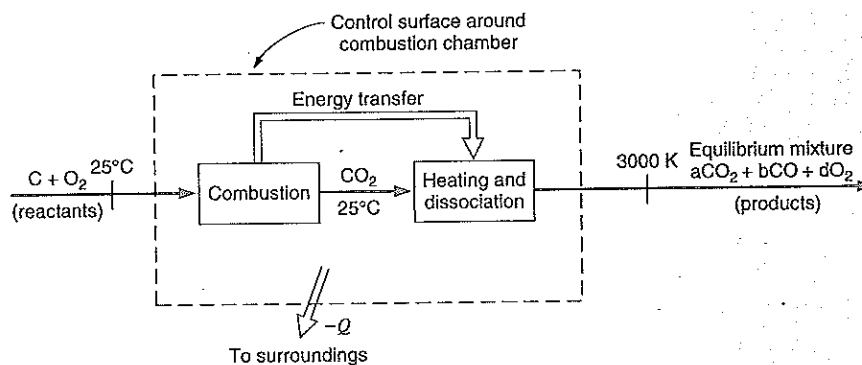
FIGURE 15.9 Sketch for Example 15.5.
