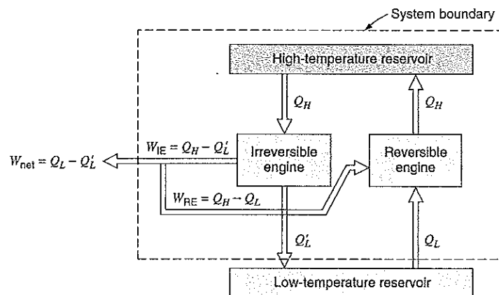
FIGURE 7.20 Demonstration of the fact that the Carnot cycle is the most efficient cycle operating between two fixed-temperature reservoirs.
