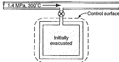
FIGURE 6.14 Flow into an evacuated vessel—control volume analysis.
