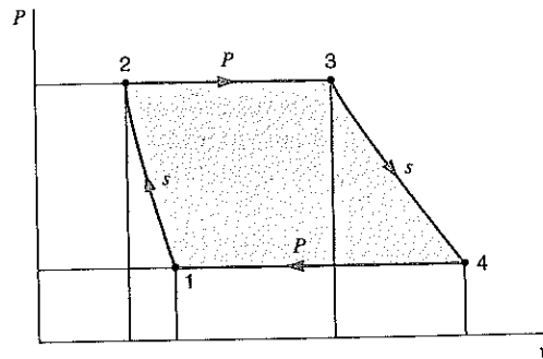
FIGURE 11.2 Four-process power cycle.
