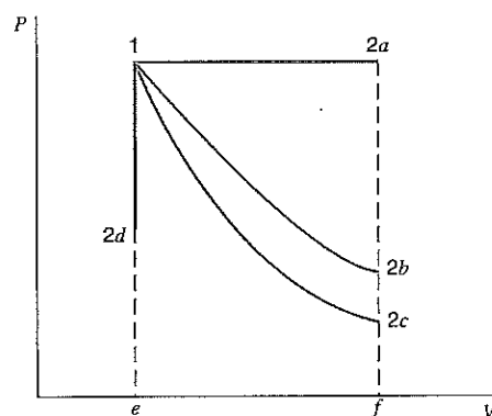
FIGURE 4.8 Pressure-volume diagram showing work done in the various processes of Example 4.1.
