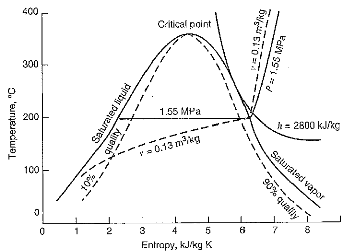
FIGURE 8.5 Temperature-entropy diagram for steam.
