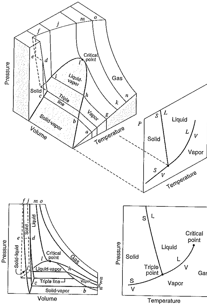
FIGURE 3.18 Pressure–volume–temperature surface for a substance that expands on freezing.
