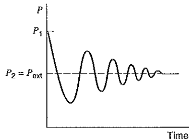
FIGURE 4.15 Cylinder pressure as a function of time.
