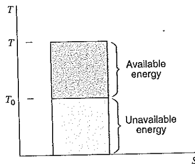
FIGURE 10.2 T - S diagram for constant-temperature energy source.
