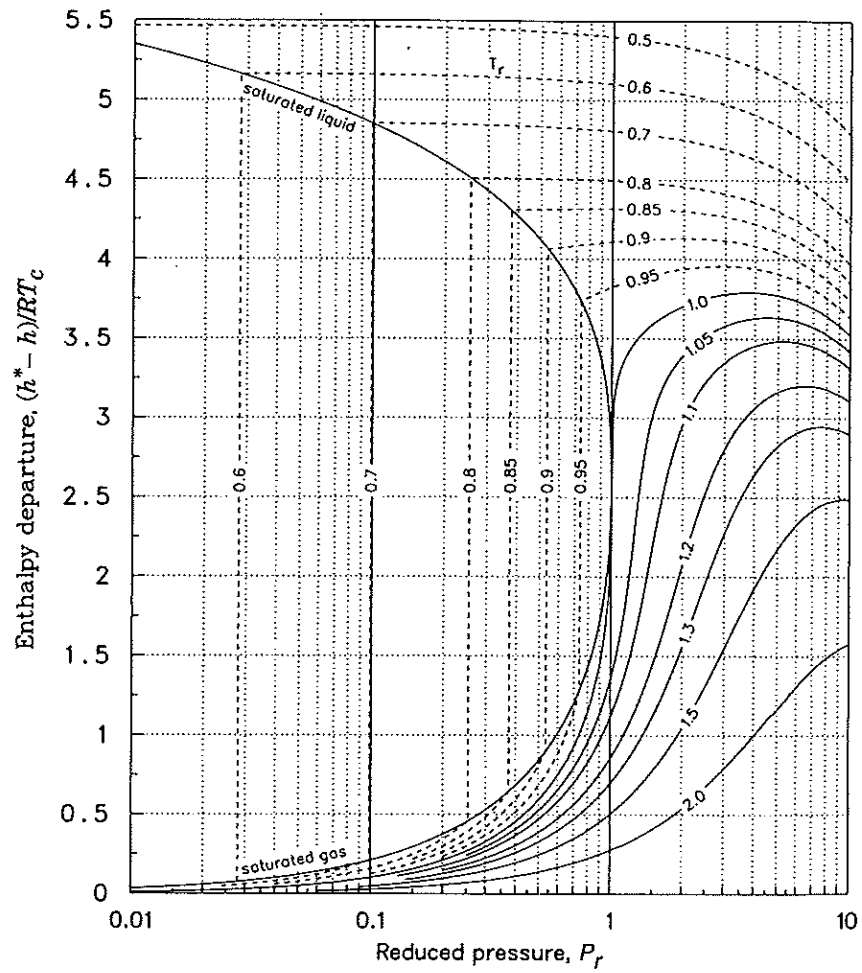
FIGURE D.2 Lee-Kesler Simple Fluid Enthalpy Departure.
