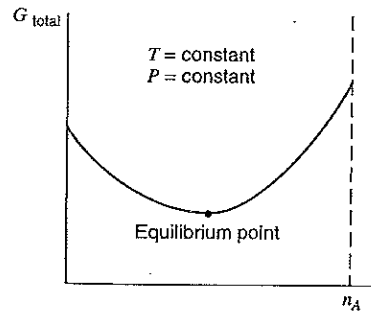
FIGURE 15.3 Illustration of the requirement for chemical equilibrium.
