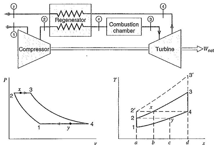
FIGURE 11.21 The ideal regenerative cycle.
