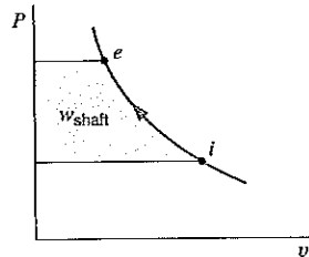
FIGURE 9.7 Shaft work from Eq. 9.18.
