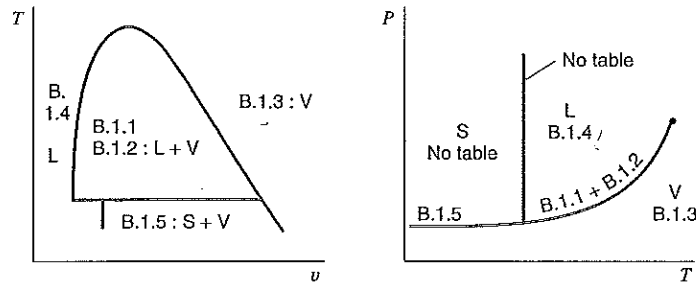
FIGURE 3.8 Listing of the steam tables.
