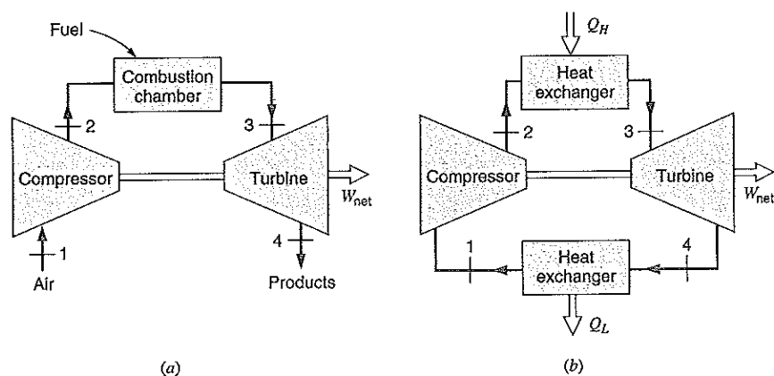
FIGURE 11.18 A gas turbine operating on the Brayton cycle. (a) Open cycle. (b) Closed cycle.
