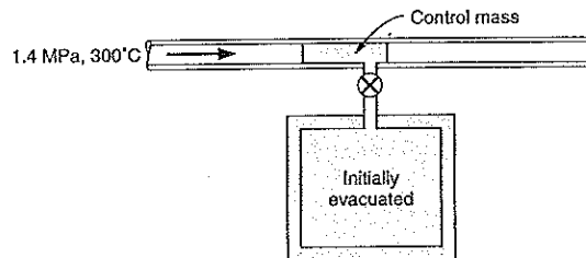
FIGURE 6.15 Flow into an evacuated vessel—control mass.
